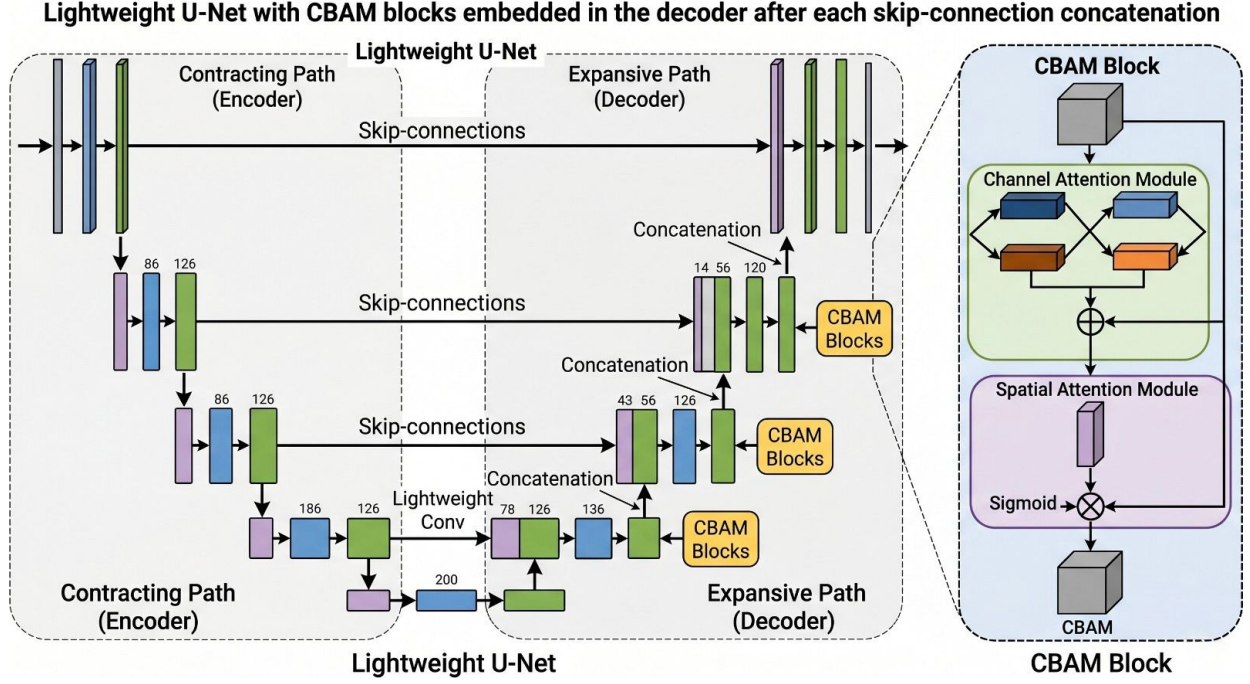
Fig. 1. Lightweight U-Net with CBAM blocks embedded in the decoder after each skip-connection concatenation.
